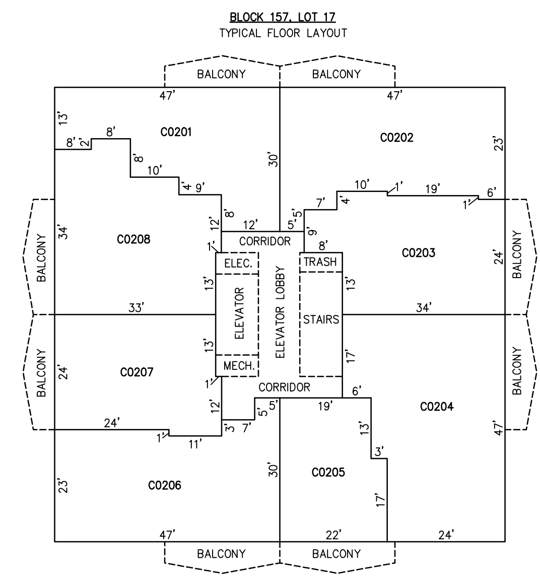
SUNSET HARBOUR CONDOMINIUM 236 NORTH DERBY AVENUE DETAIL "A" SCALE: 1"=20'
