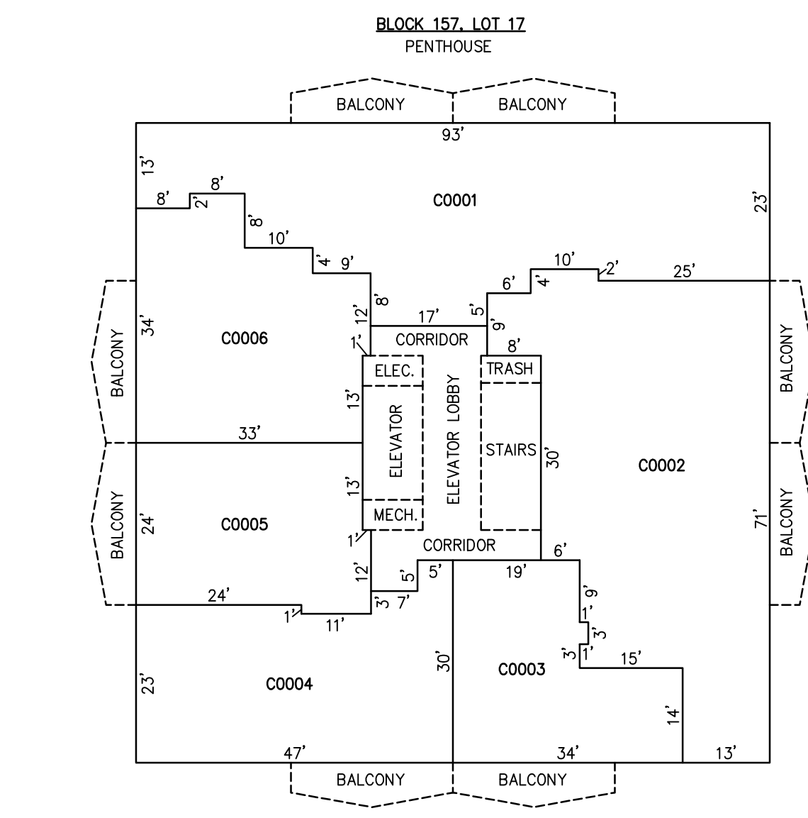
SUNSET HARBOUR CONDOMINIUM 236 NORTH DERBY AVENUE DETAIL "A" SCALE: 1"=20'
