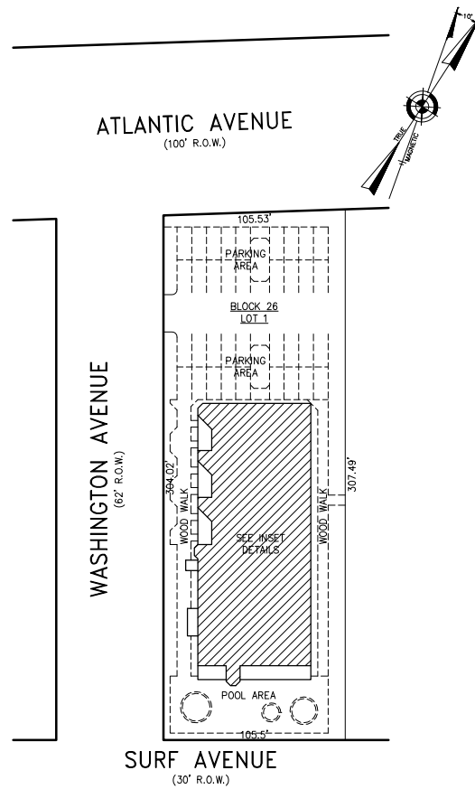
PLAN SCALE: 1"=50'
