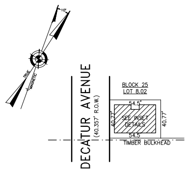
PLAN SCALE: 1"=50'
