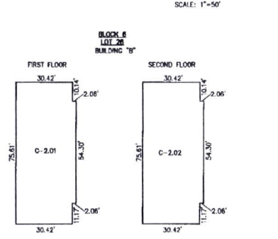
PLAN SCALE: 1"=50'
