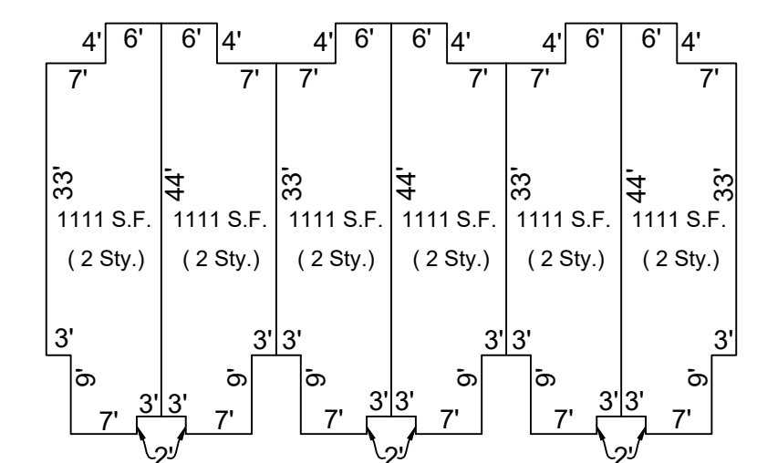
UNIT A Scale : 1" = 20'
