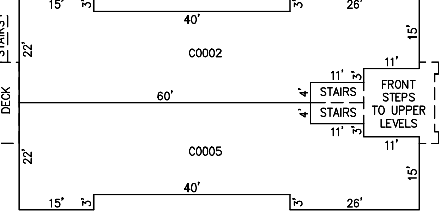
THIRD FLOOR
