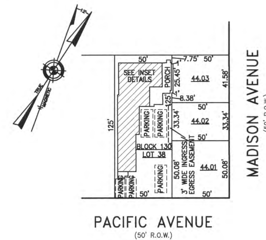
PLAN SCALE: 1"=50'
