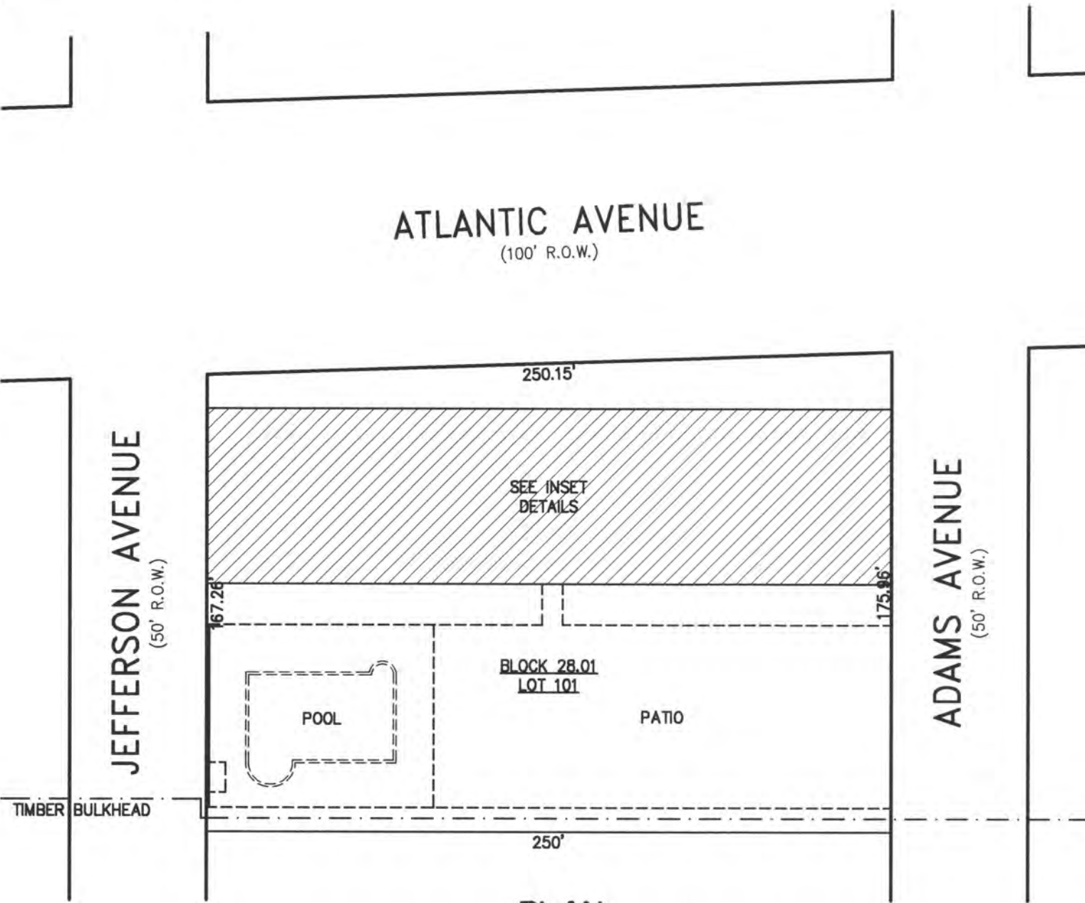
PLAN SCALE: 1"=50'
